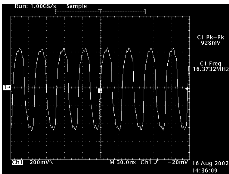
Figure 17: GPS 16.368 MHz reference clock from TCXO at J009
