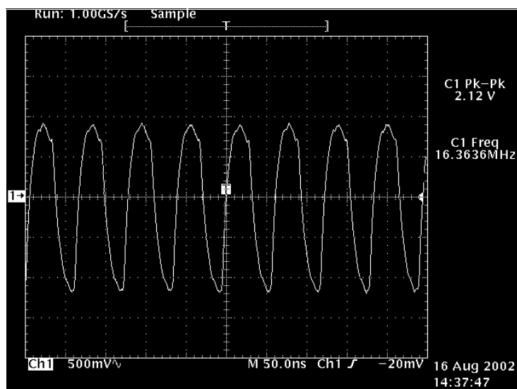
Figure 18: GPS 16.368 MHz reference clock to GPS BB
